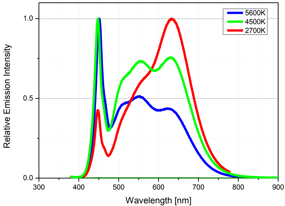
Fig 1. Color Spectrum, I_F = 100\text{mA} , T_a = 25^\circ\text{C} , RH30%
